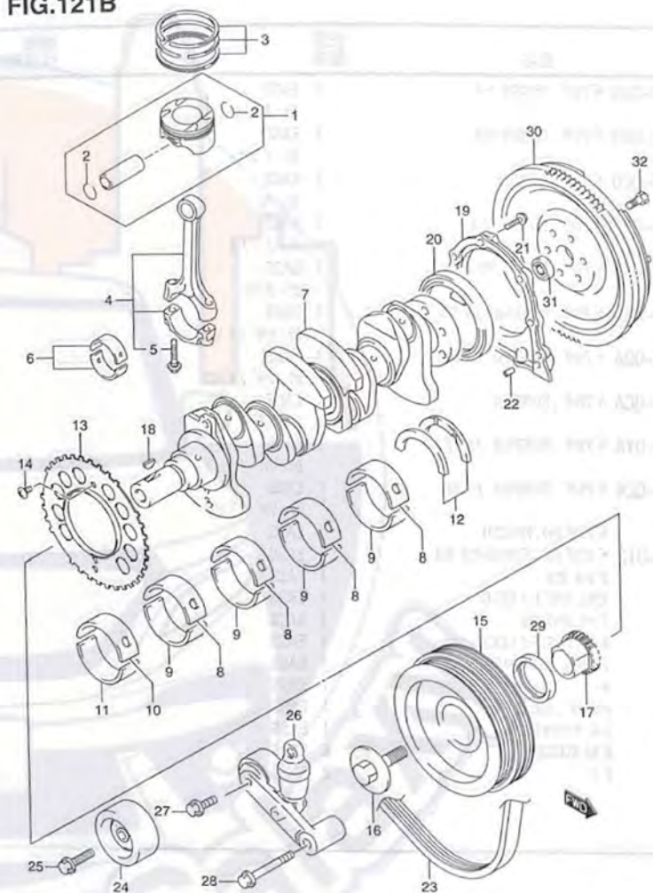
MA36S-2 121B CRANKSHAFT (2)
