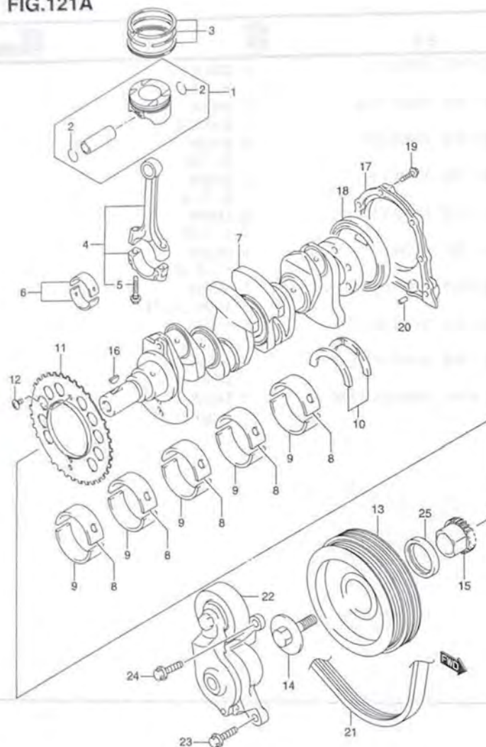
MA36S-2 121A CRANKSHAFT (1)
