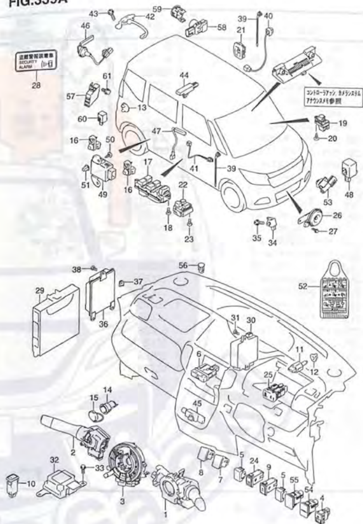
MA36S-2 339A ELECTRICAL CONTROL (1)
