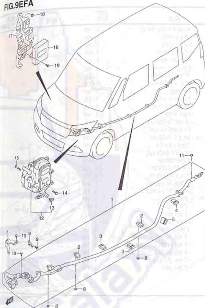
MA36S-2 9EFA DRIVE MOTOR HARNESS
