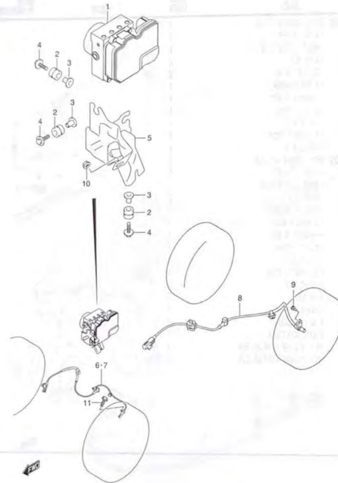
MA36S-2 561A ANTI LOCK BRAKE SYSTEM (1)
