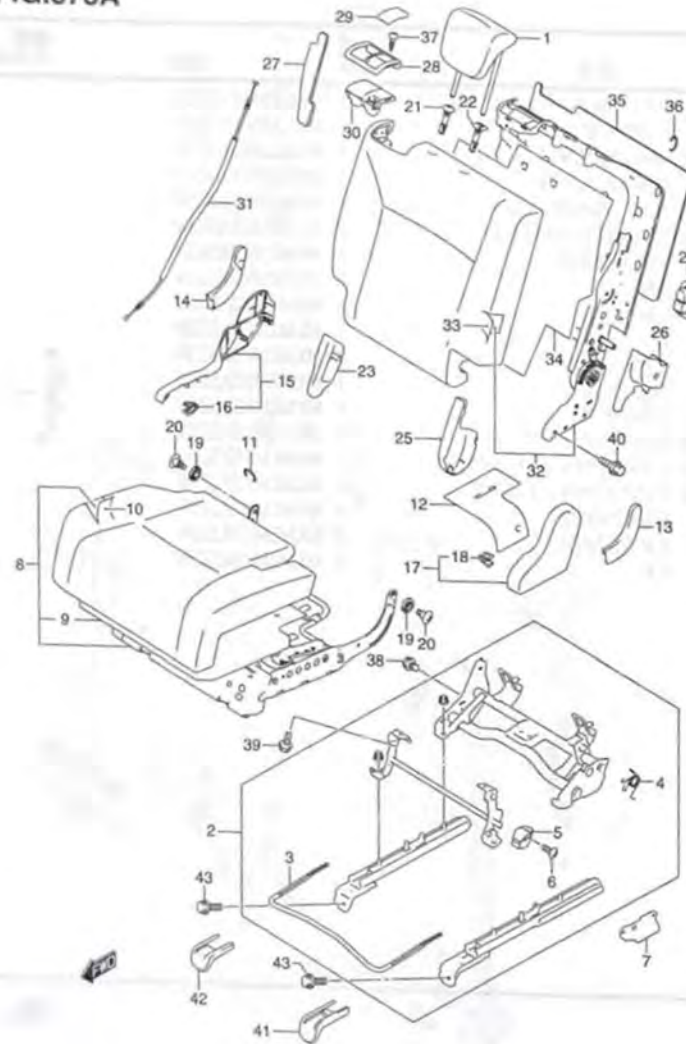
MA36S-2 875A REAR RH SEAT (1)
