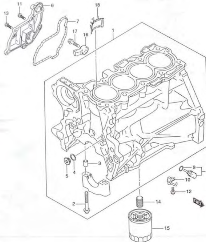
MA36S-2 112A CYLINDER
