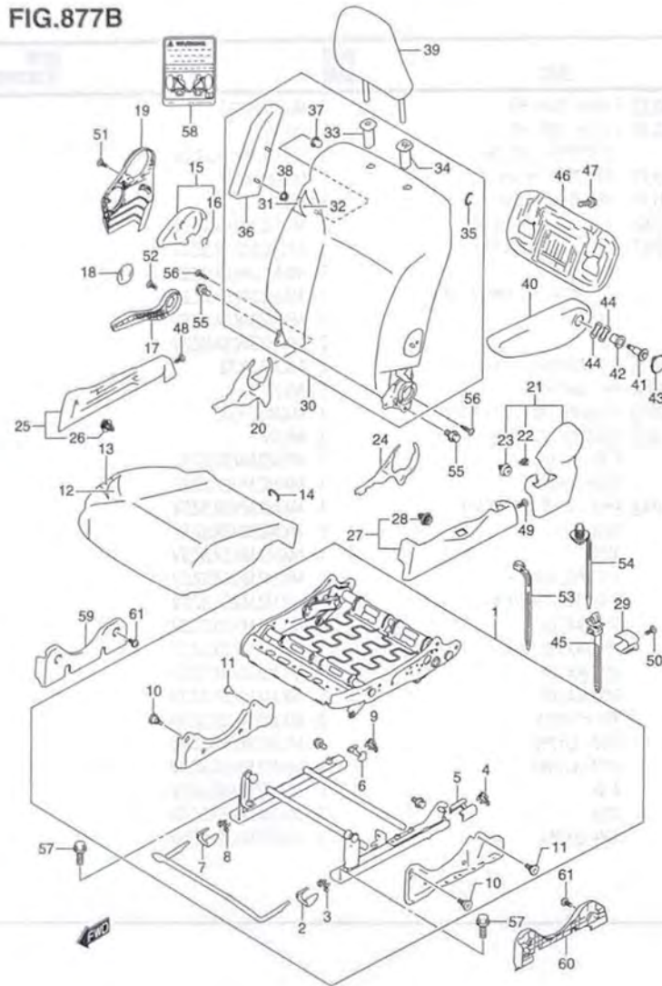
MA36S-2 877B FRONT RH SEAT (2)
