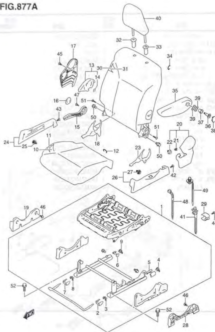
MA36S-2 877A FRONT RH SEAT (1)
