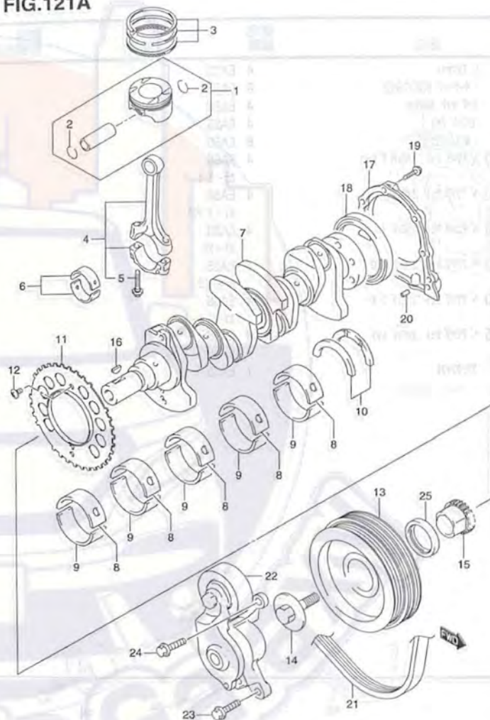
MA36S-2 121A CRANKSHAFT (1)
