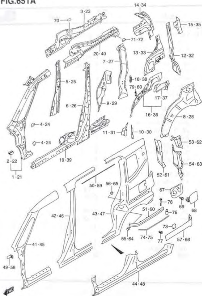
MA36S-2 651A SIDE BODY PANEL
