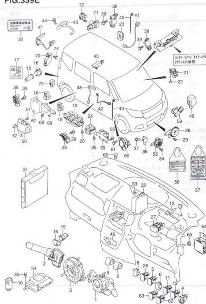
MA36S-2 339E ELECTRICAL CONTROL (5)
