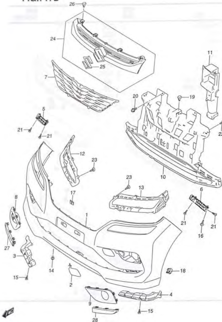
MA36S-2 717D FRONT BUMPER (4)
