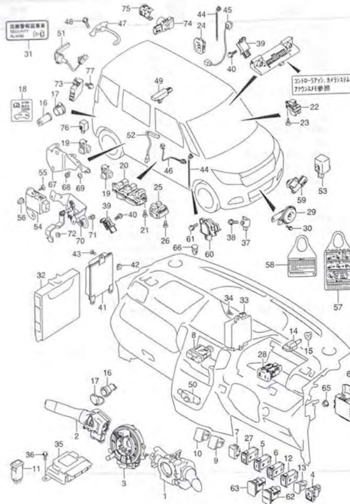
MA36S-2 339B ELECTRICAL CONTROL (2)
