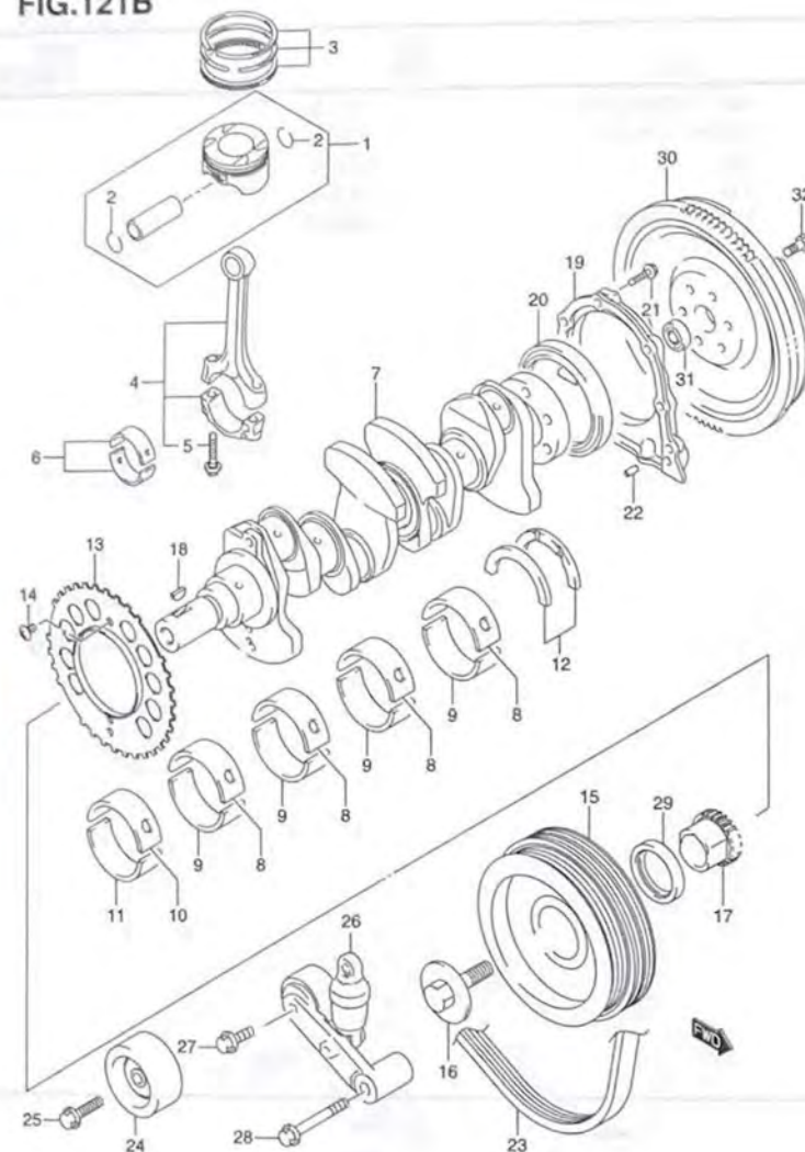
MA36S-2 121B CRANKSHAFT (2)
