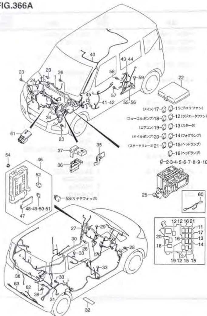
MA36S-2 366A WIRING HARNESS (1)
