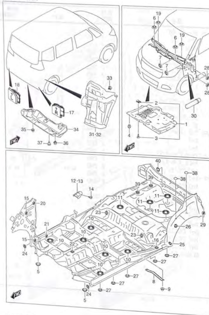
MA36S-2 676A COVER/CAP (1)
