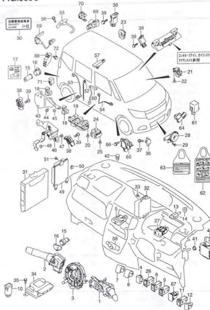
MA36S-2 339C ELECTRICAL CONTROL (3)
