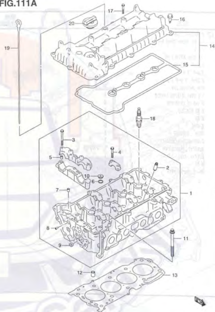
MA36S-2 111A CYLINDER HEAD
