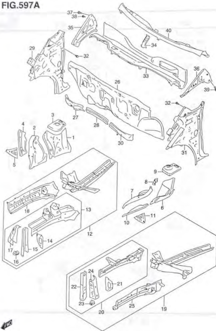
MA36S-2 597A FRONT BODY PANEL
