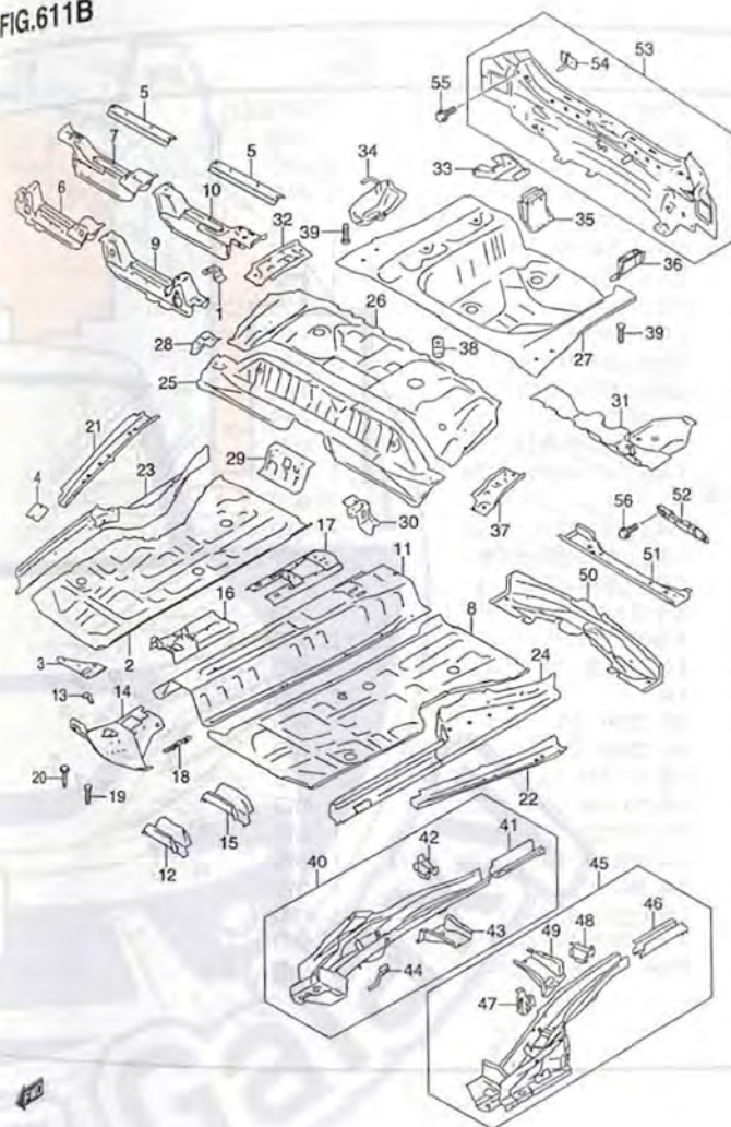
MA36S-2 611B FLOOR PANEL (2)
