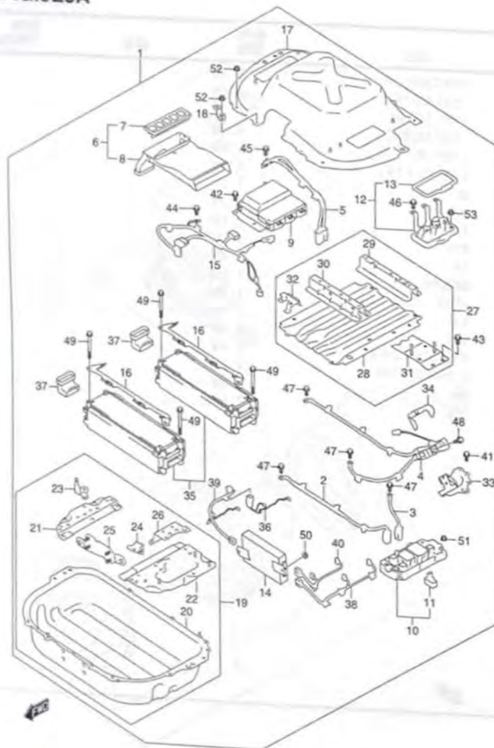
MA36S-2 9EJA DRIVE MOTOR BATTERY
